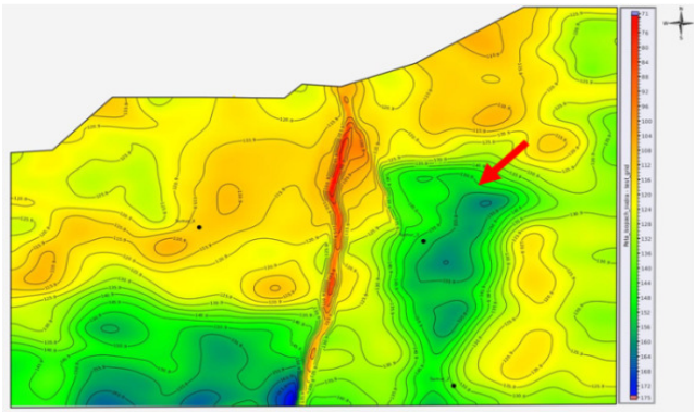
Figure 10 Gross isopach maps, depth maps iso results grid structure over the depth map layer MMC and MMC under a layer structure
