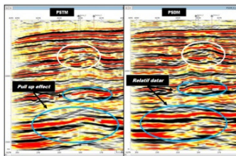
Comparison of PSTM and PSDM section
