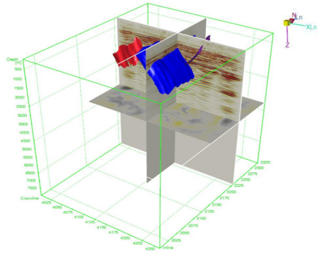
Figure 8 Three faults were identified in reseach area, SBI field, North West Java basin. The third fault included normal faults)
