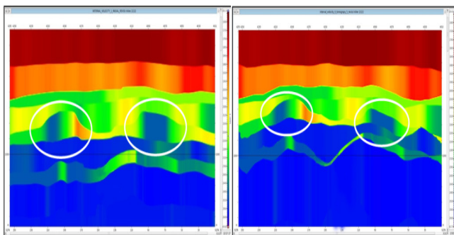
Figure 4 Interval velocity model results from dix transform, before tomography (left) and after tomography process (right)
