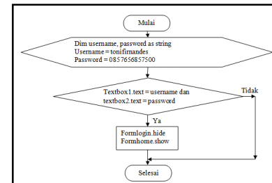
Gambar 3.12 Diagram Alir Form Login
