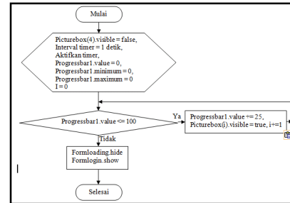
Gambar 3.11 Diagram Alir Algoritma Form Loading
