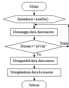
Gambar 3.15 Diagram Alir Program Arduino Node Slave 1
