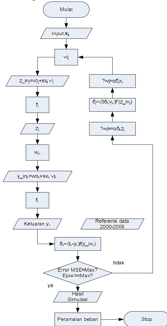
Gambar 3.1. Flowchart [7]
