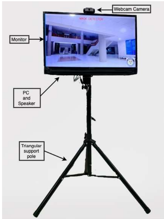
Face-mask detection
