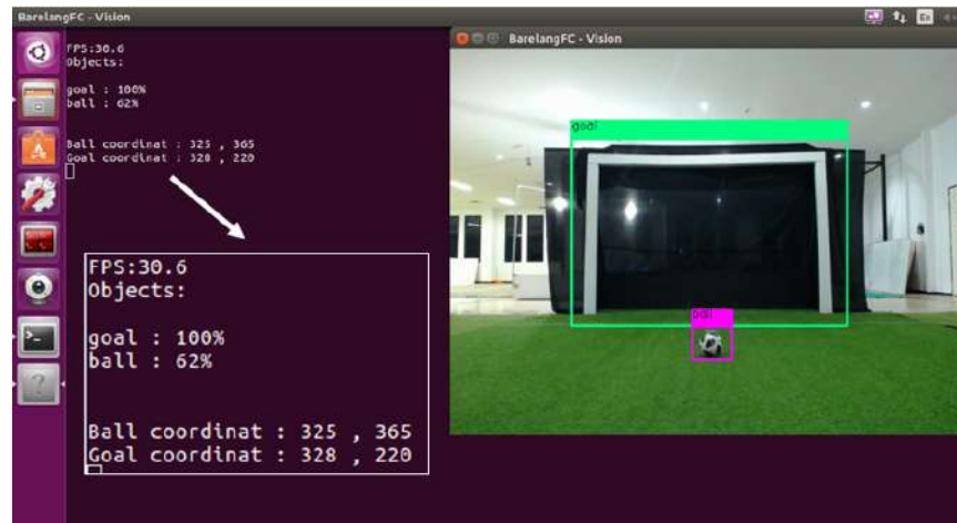
Object detection
