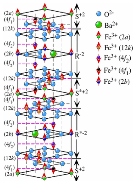
Gambar 2. Struktur kristal BaFe_{12}O_{19} (Ümit, 2009)
